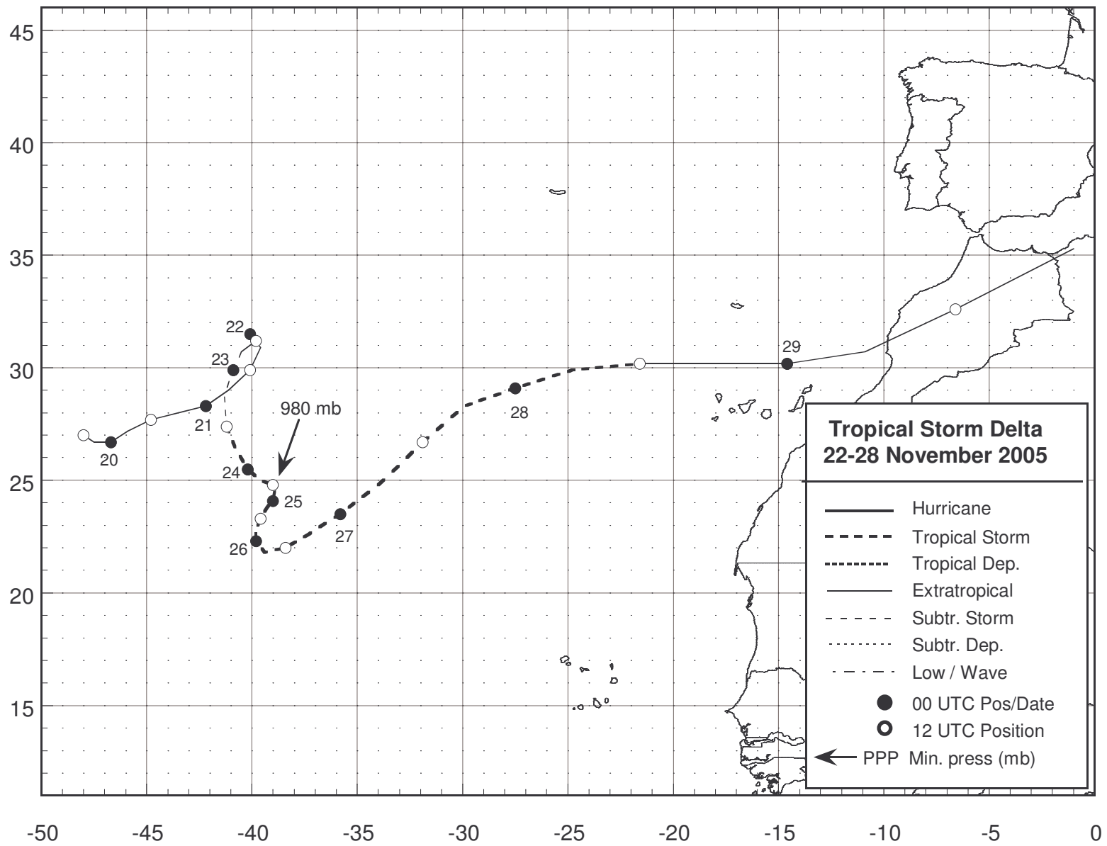
Figure 1. Best track positions for Tropical Storm Delta, 22 - 28 November 2005.
