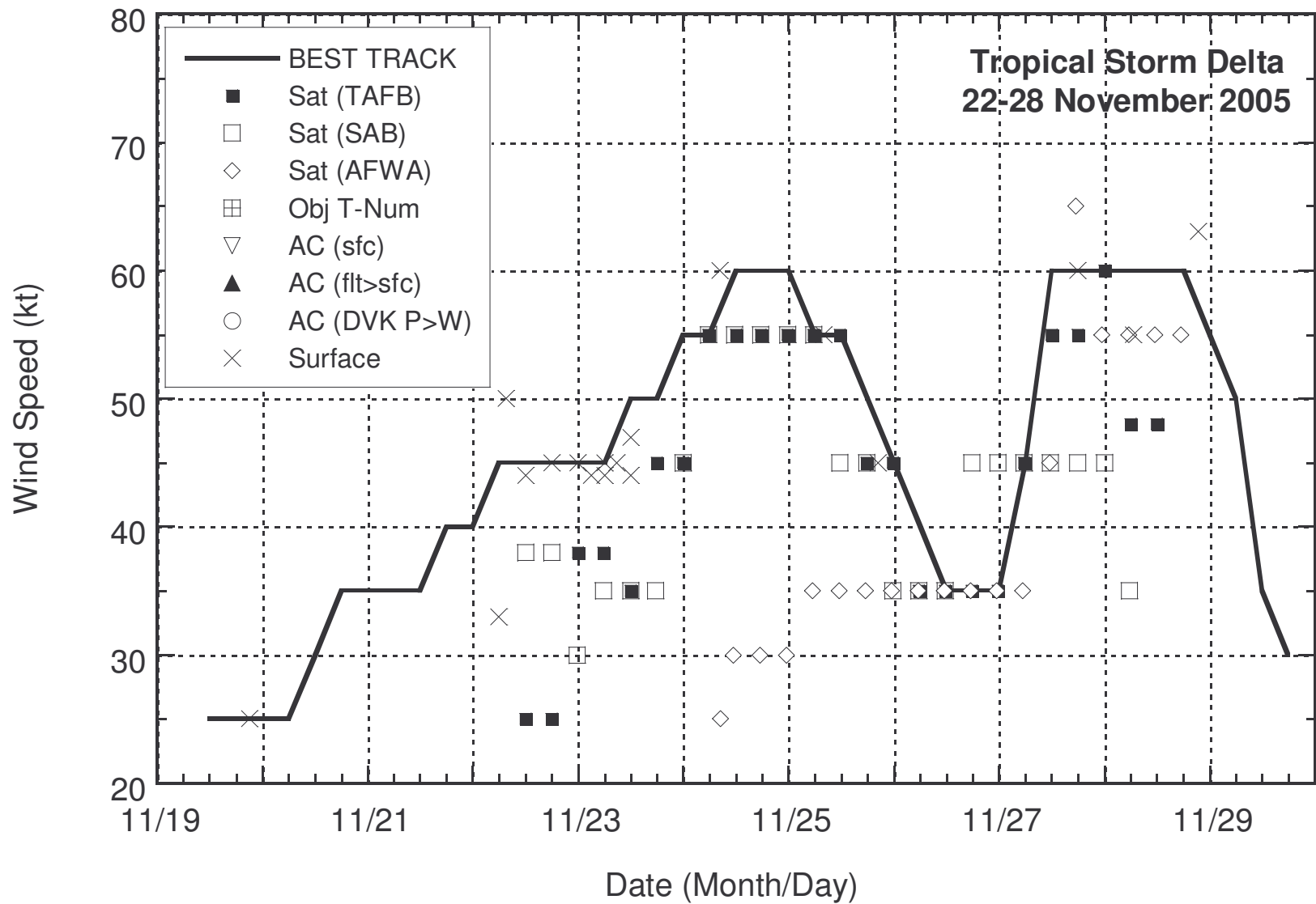
Figure 2. Selected wind observations and best track maximum sustained surface wind speed curve for Tropical Storm Delta, 22 - 28 November 2005.
